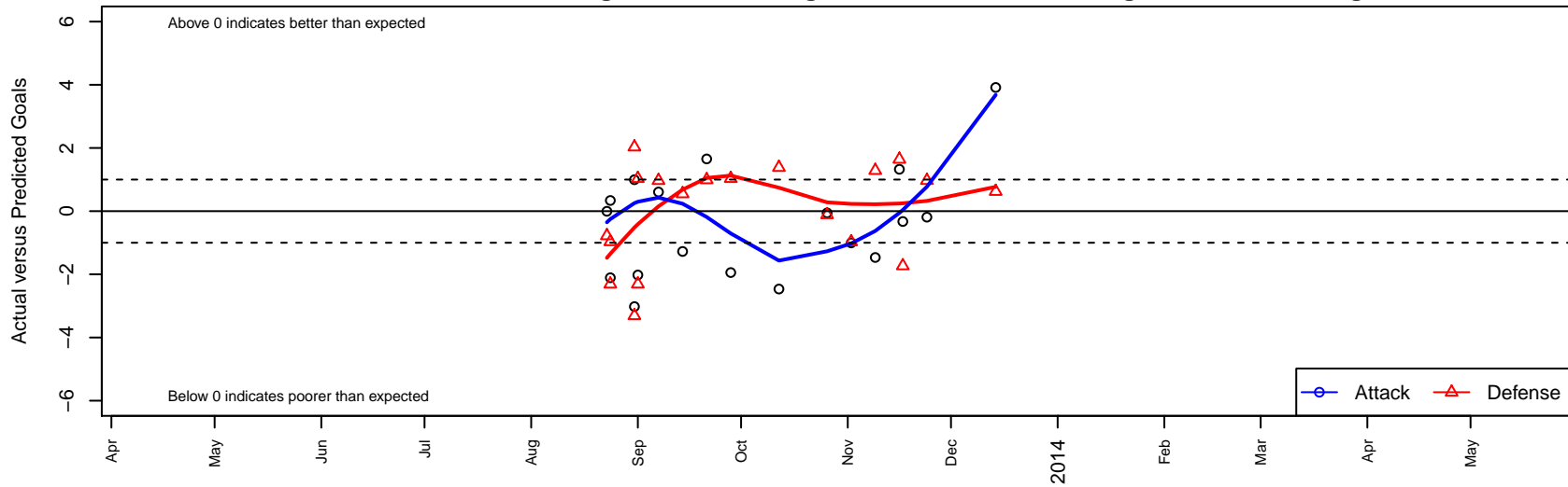
Tynecastle FC-R B01 Dots are actual minus expected GF (blue circles) and GA (red triangles). Blue line is smoothed change in attack strength. Red is smoothed change in defense strength.
